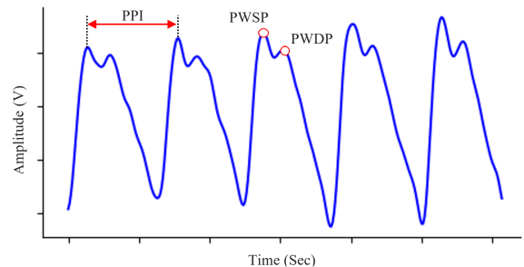
Fig. 1. BVP signal (PPI: Peak to Peak Interval, PWSP: Pulse Wave Systolic Peak, PWDP: Pulse Wave Diastolic Peak )
